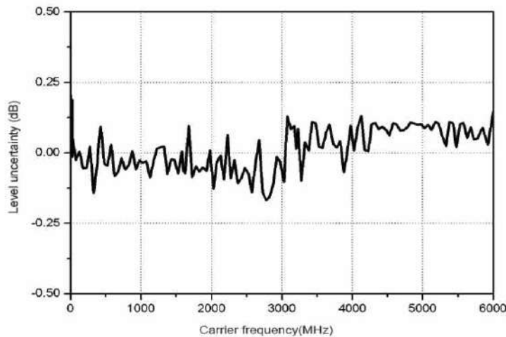
Measured -60dBm output level VS frequency
