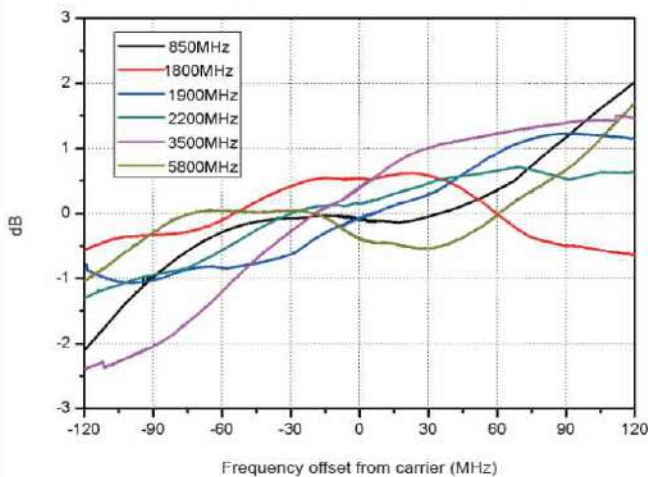
Measured external IQ bandwidth
