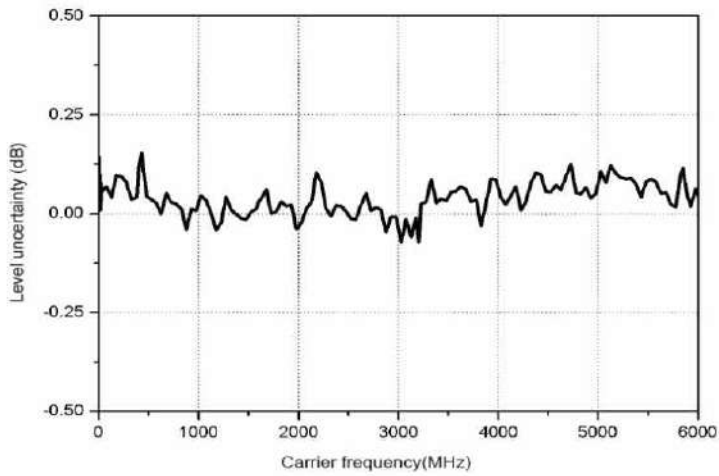
Measured +13dBm output level VS frequency
