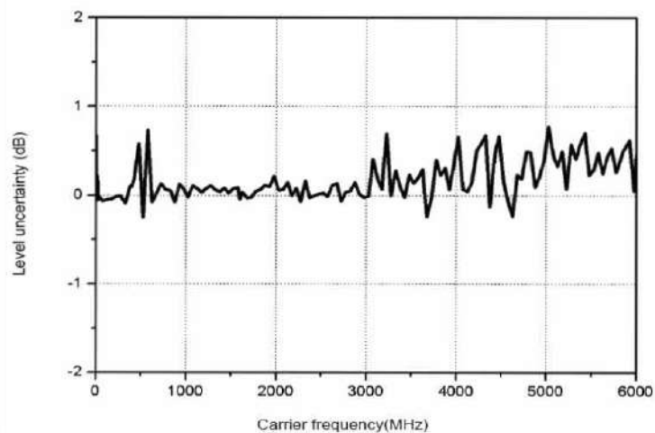
Measured -127dBm output level VS frequency
