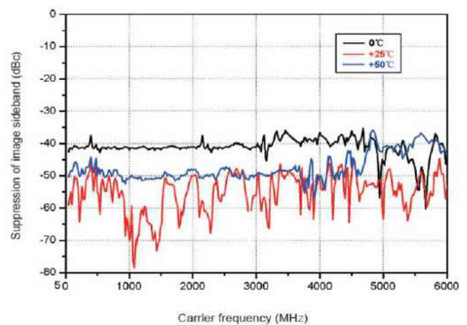
Measured suppression of image sideband
