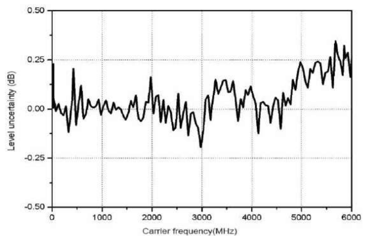
Measured -110dBm output level VS frequency
