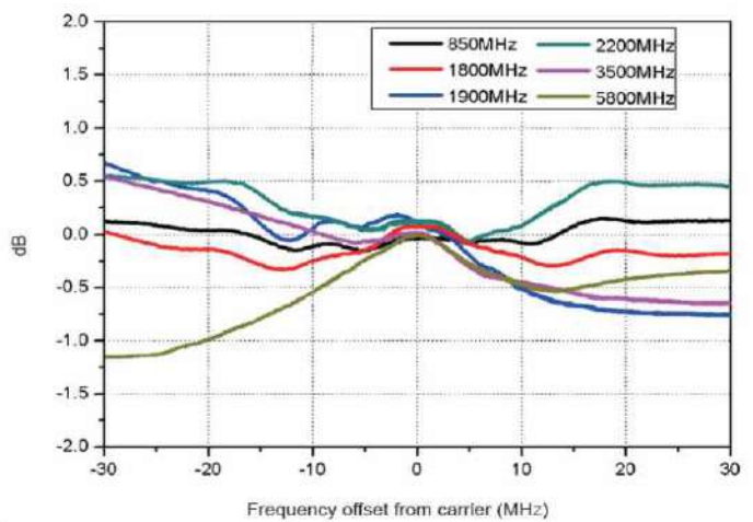
Measured internal IQ bandwidth
