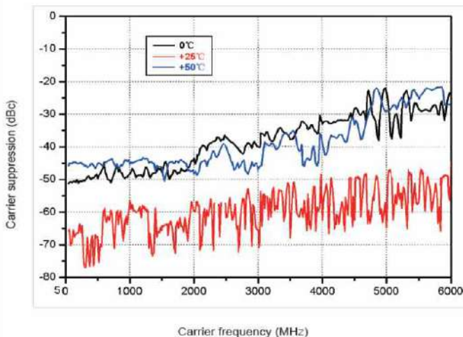
Measured carrier suppression
