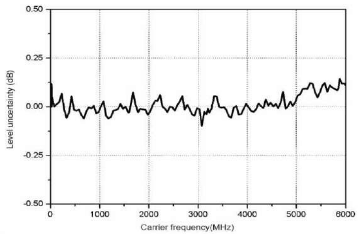
Measured 0dBm output level VS frequency
