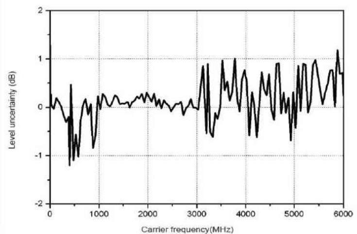
Measured -136dBm output level VS frequency
